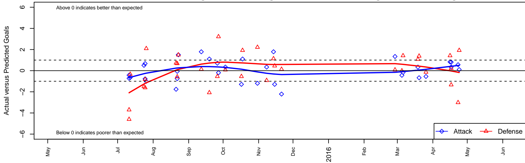
Impact FC Black B02 Dots are actual minus expected GF (blue circles) and GA (red triangles). Blue line is smoothed change in attack strength. Red is smoothed change in defense strength.
